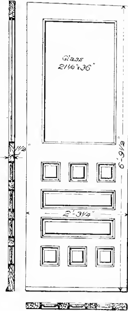
Figs. 1784-1786. END DOOR OF COACH. NORFOLK & WESTERN RAILROAD.
